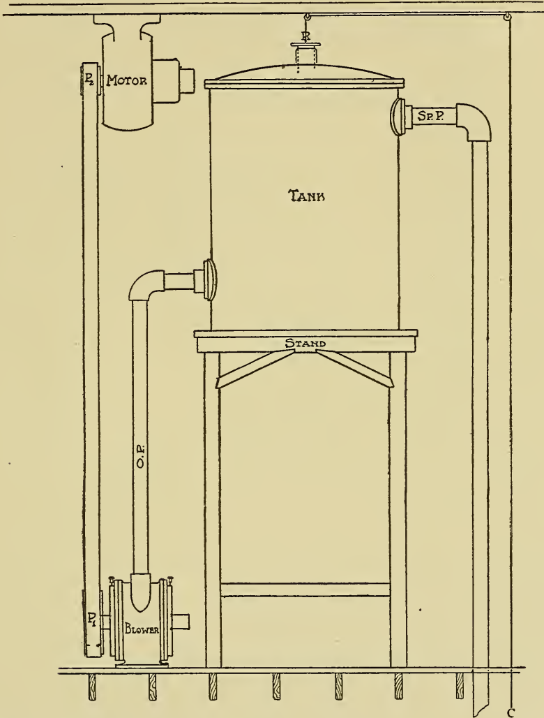
FIG. 9. SYSTEM OF INSTALLING BLOWER, MOTOR, AND AIR TANK
